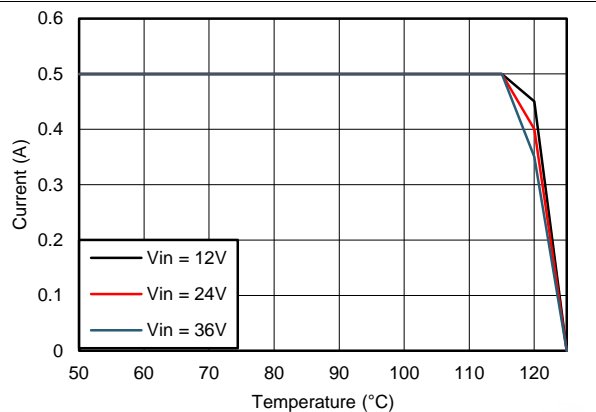
V_{OUT} = 5\text{ V} F_S = 200\text{ kHz} R_{\theta JA} = 20^\circ\text{C/W}
