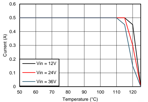
V_{OUT} = 3.3\text{ V} F_S = 500\text{ kHz} R_{\theta JA} = 20^\circ\text{C/W}
