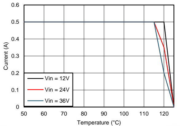
V_{OUT} = 5\text{ V} F_S = 500\text{ kHz} R_{\theta JA} = 20^\circ\text{C/W}
