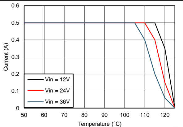
V_{OUT} = 5\text{ V} F_S = 1\text{ MHz} R_{\theta JA} = 20^\circ\text{C/W}
