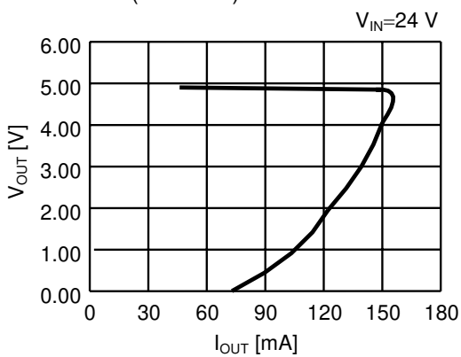
S-8750xxx Series ( T_a=25^\circ\text{C} )
