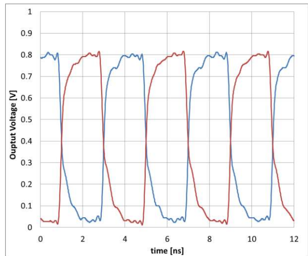
Figure 20. 250MHz HCSSL
