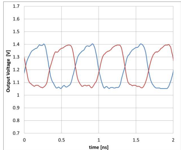
Figure 18. 1.5GHz LVDS
