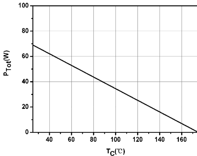
Fig.7-Power Derating
