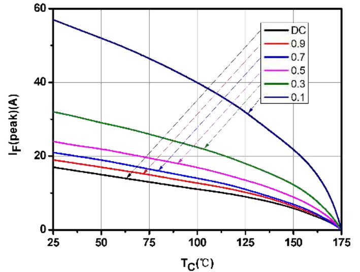
Fig.8-Current Derating
