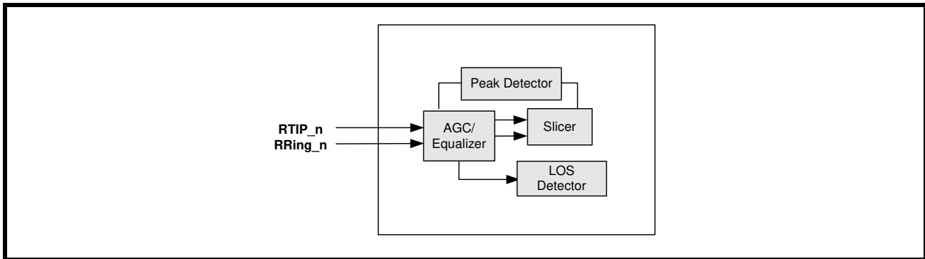
FIGURE 7. ACG/EQUALIZER BLOC DIAGRAM
