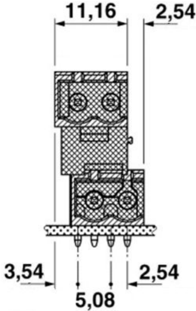
Dimensioned drawing
