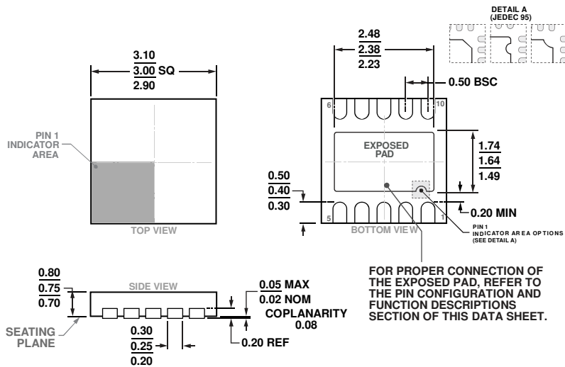
Figure 46. 10-Lead Lead Frame Chip Scale Package [LFCSPP] 3 mm x 3 mm Body and 0.75 mm Package Height (CP-10-9) Dimensions shown in millimeters
