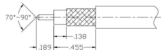
RECOMMENDED CABLE STRIPPING DIMENSIONS
