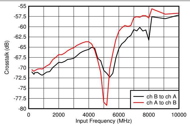
Figure 6-2. Crosstalk vs Input Frequency
