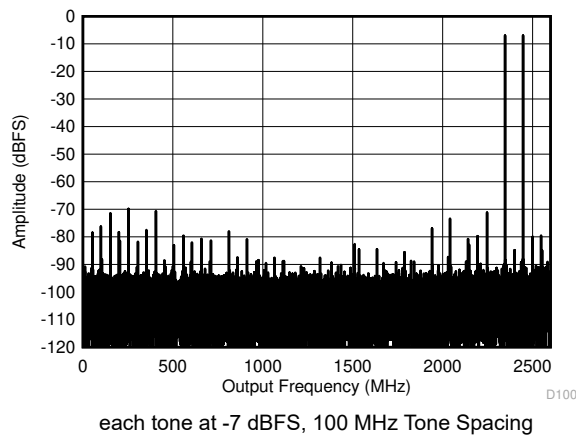
Figure 6-25. Dual Channel Mode: Two Tone FFT at 2397 MHz
