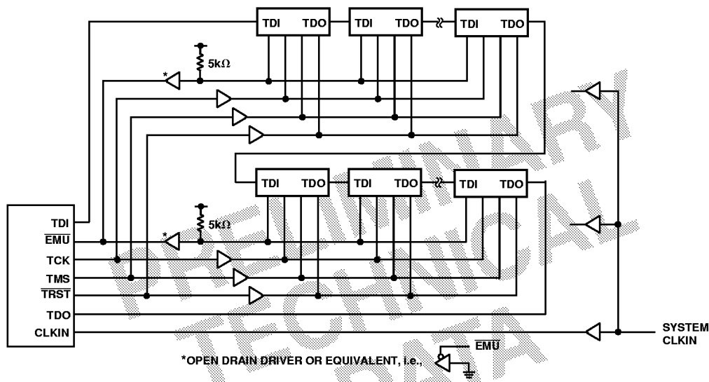
Figure 7. JTAG Clocktree for Multiple ADSP-2106x Systems
