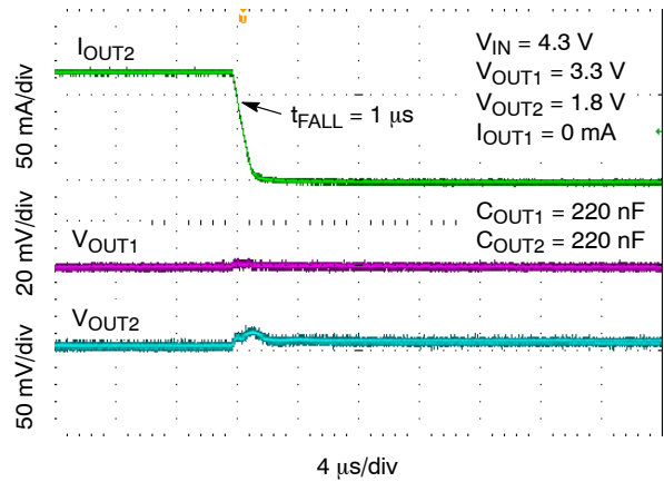
Figure 38. Load Transient Response – Falling Edge, I_{OUT} = 130 \text{ mA} to 0.1 \text{ mA}
