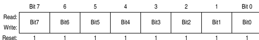
Figure 16-8. TIM Counter Modulo Low Register (TMODL)
