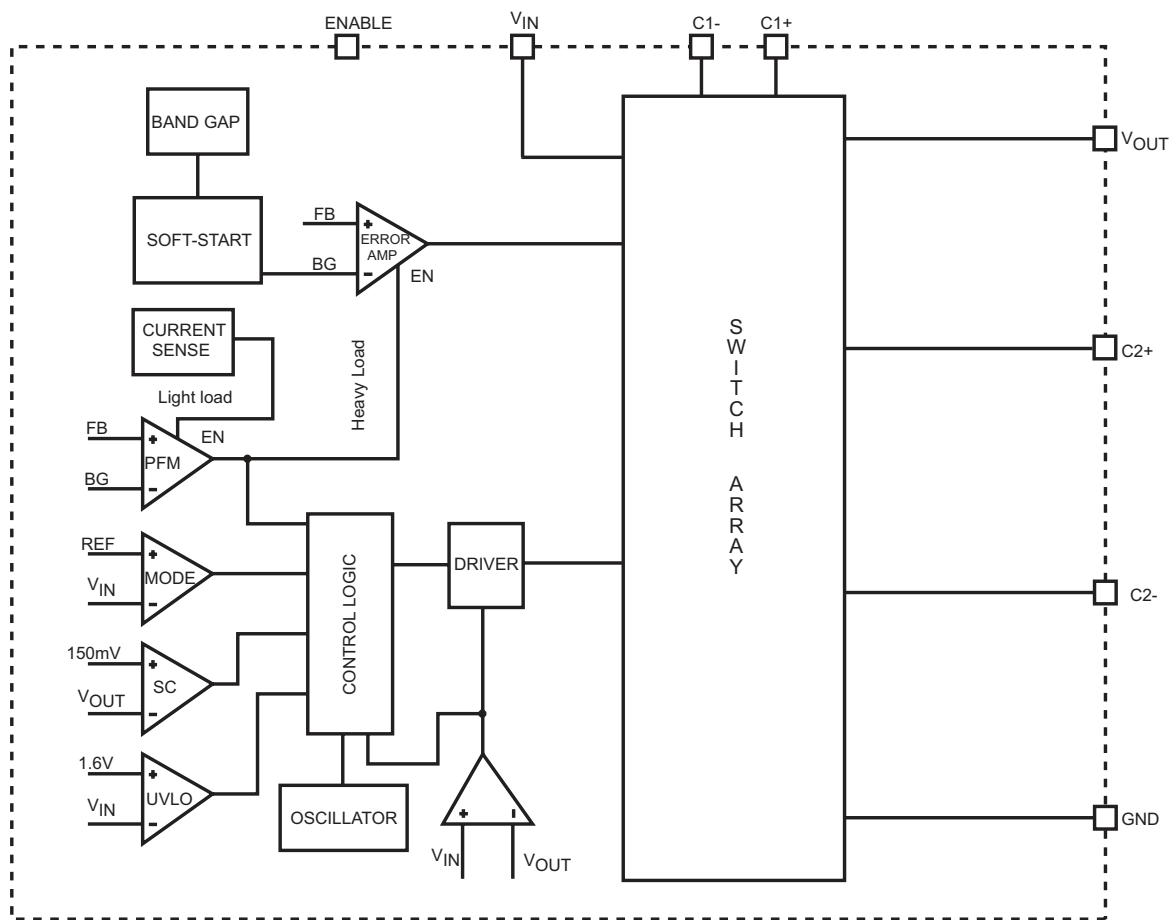
Figure 3. Block Diagram
