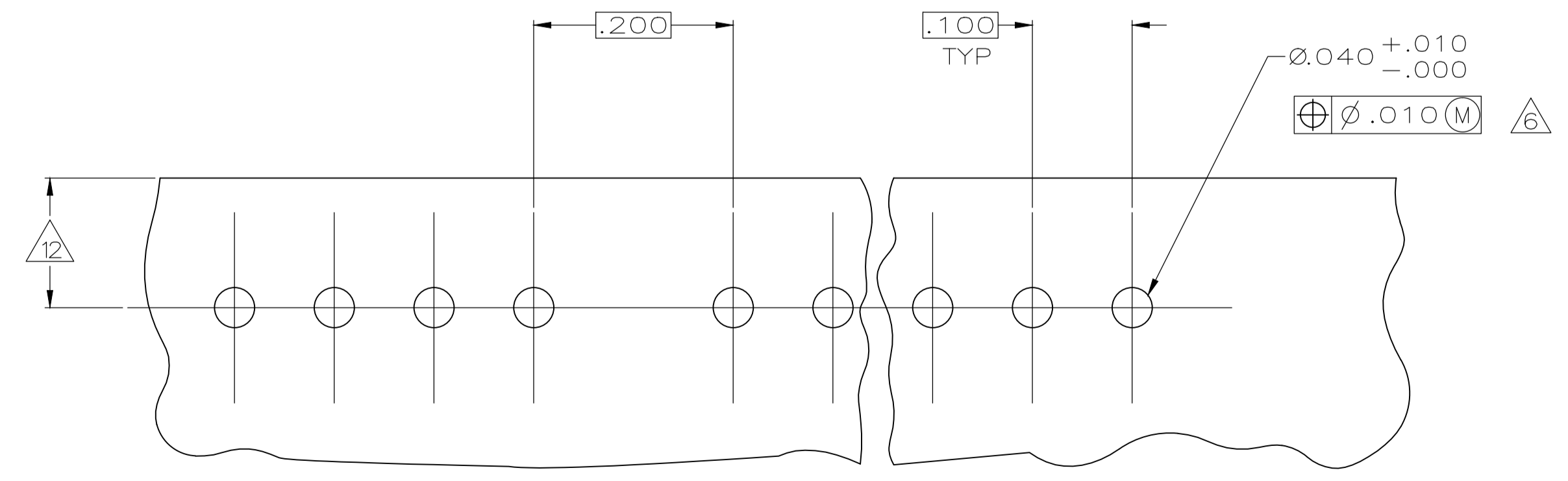
RECOMMENDED MOUNTING HOLE PATTERN 2 FOR .063 THICK P.C. BOARD
