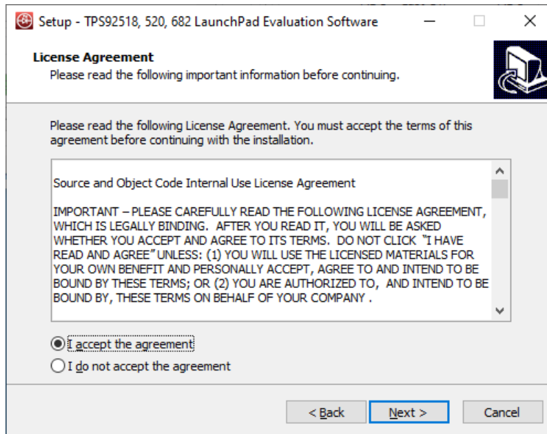
Figure 5-2. Setup Screen 2
