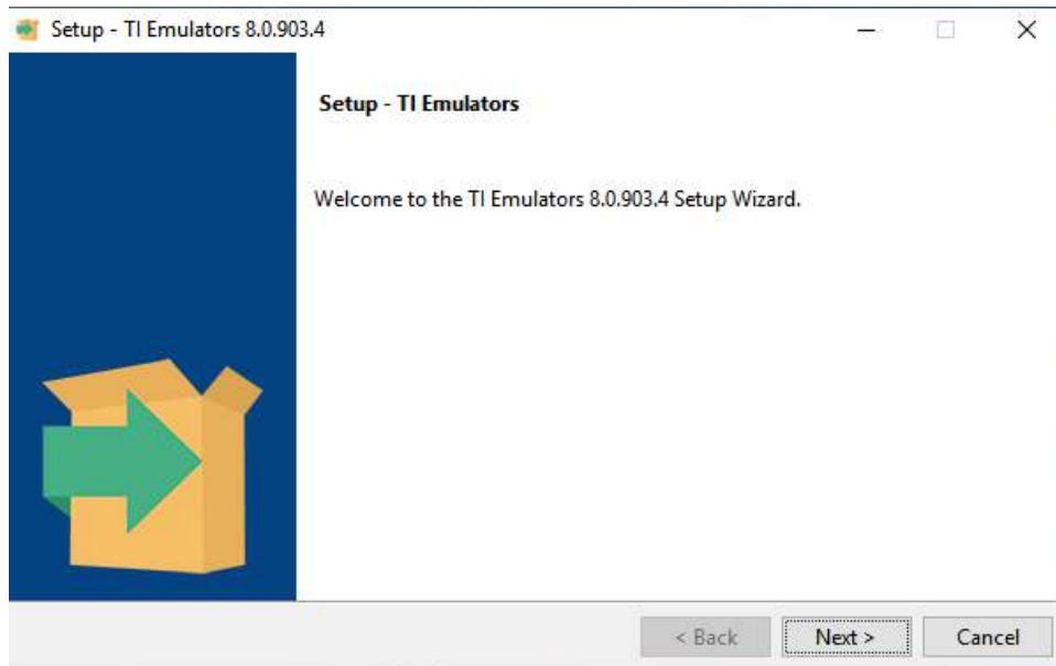
Figure 5-9. Setup Screen 9
