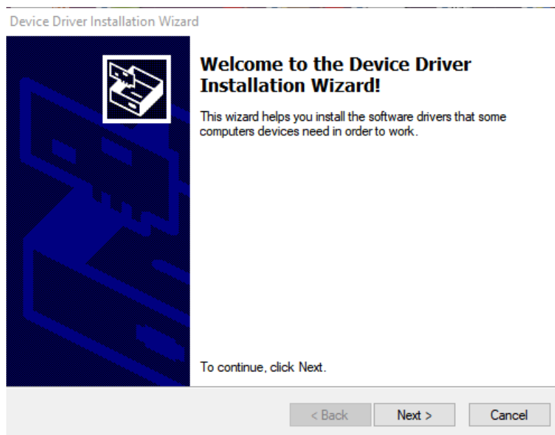
Figure 5-7. Setup Screen 7
