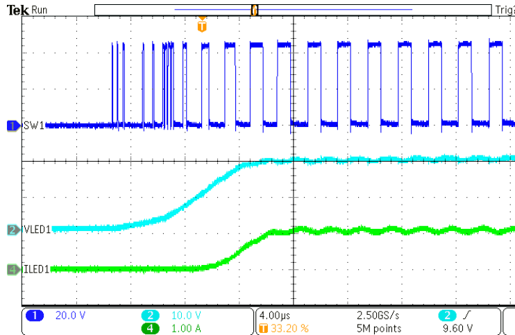
Figure 3-3. Soft-Start Waveforms
