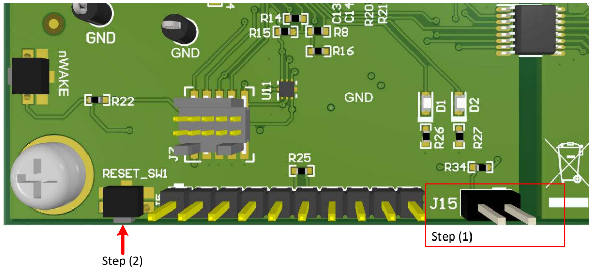
Figure 5-26. 15 Jumper and RESET_SW1 Switch for Normal Mode
