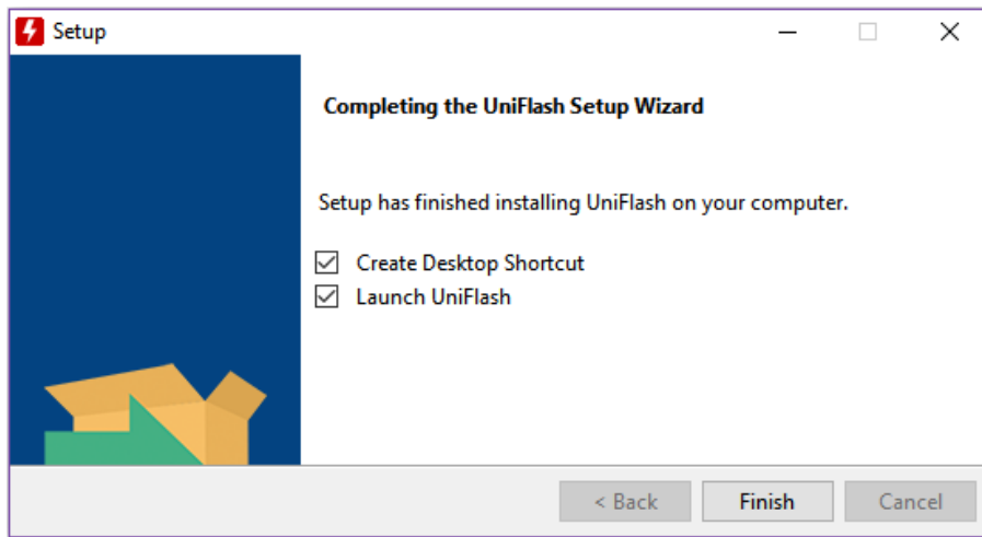
Figure 5-17. Setup Screen 17
