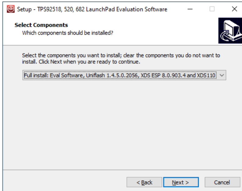
Figure 5-3. Setup Screen 3
