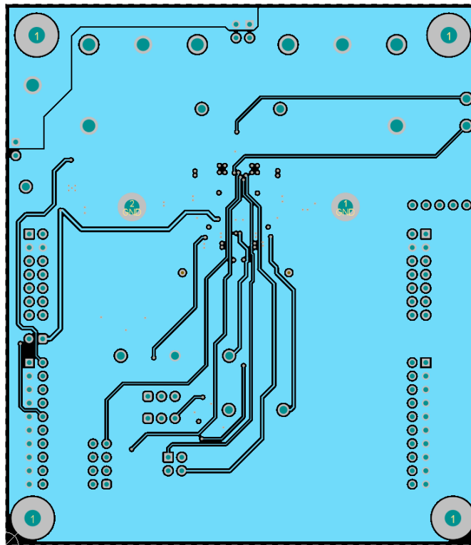
Figure 4-6. TPS92520EVM-133 Inner-Layer 2
