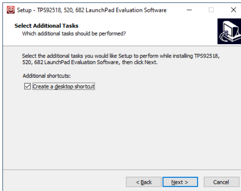
Figure 5-6. Setup Screen 6
