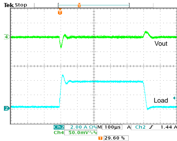
Figure 19. Load Transient at FFCM Mode
