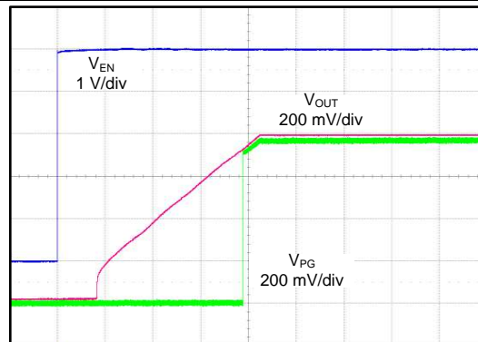
Time (2 \text{ms}/\text{div} )
