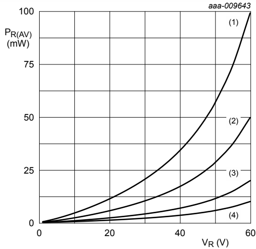
T_j = 150^\circ\text{C} (1) \delta = 1 (2) \delta = 0.5 (3) \delta = 0.2 (4) \delta = 0.1
