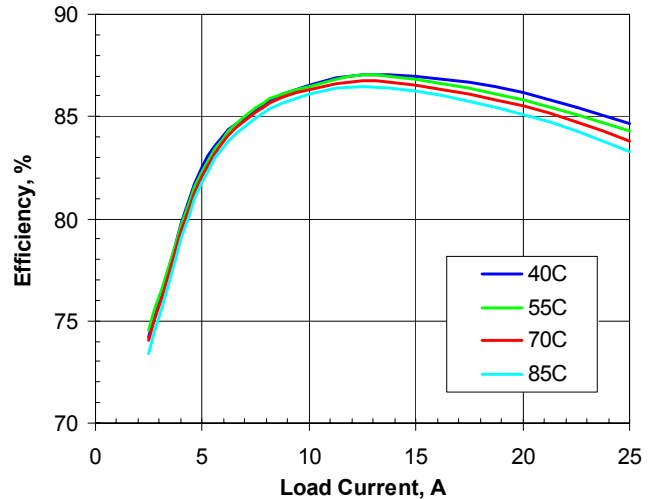
Figure 3. Efficiency vs. load current and ambient temperature for SSQE48T25015 converter mounted vertically with Vin=48V and air flowing from pin 1 to pin 3 at a rate of 200LFM (1.0m/s).
