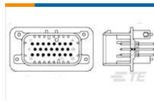
TE Part #1-776230-1 35POS,PIN DIA 1.3,HDR ASSY, 180DEG,COD 1
