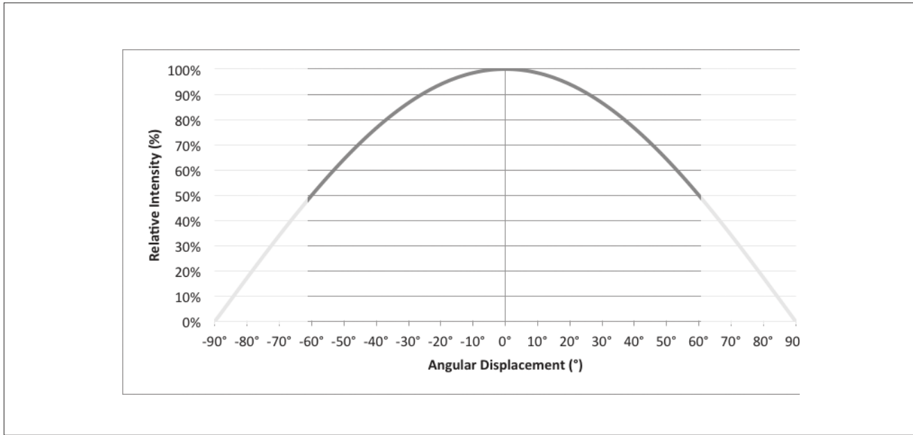
Figure 18: Typical Spatial Radiation Pattern
