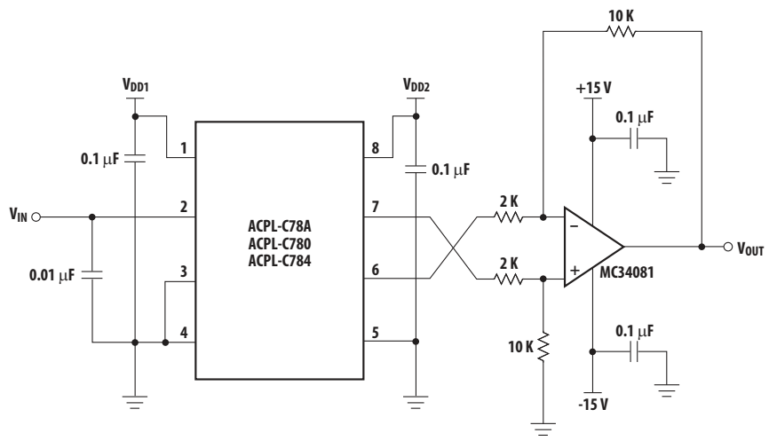
Figure 15: Propagation Delay Test Circuits
