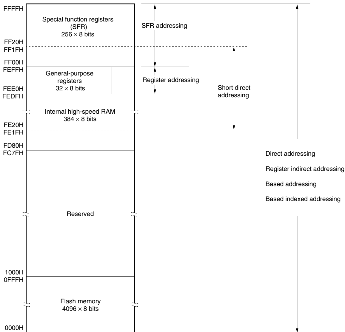
Figure 3-5. Correspondence Between Data Memory and Addressing (μPD78F0550, 78F0555, 78F0560, 78F0565)
