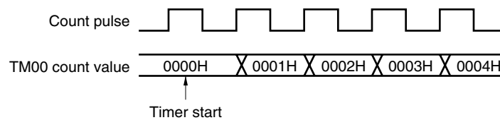
Figure 6-56. Start Timing of TM00 Count
