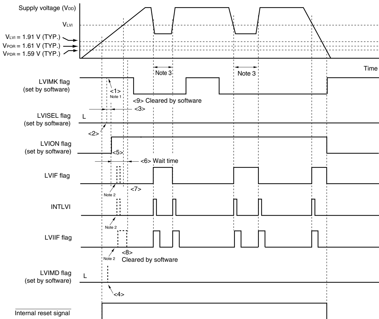
<R> Figure 22-9. Timing of Low-Voltage Detector Interrupt Signal Generation (Bit: LVISEL = 0, Option Byte: LVISTART = 1)
