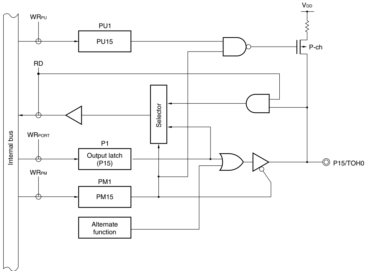
Figure 4-9. Block Diagram of P15
