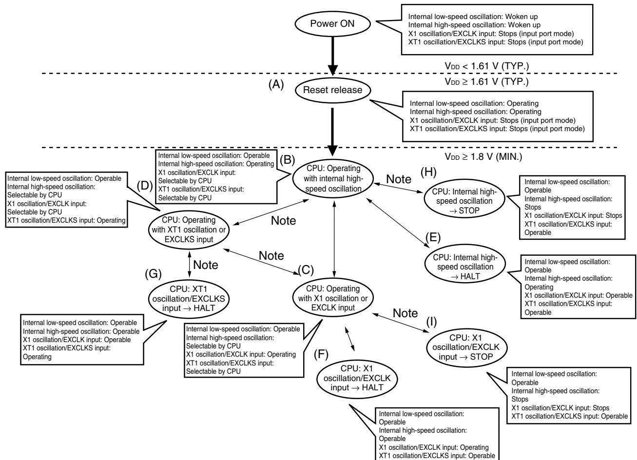
Figure 5-19. CPU Clock Status Transition Diagram (When LVI Default Start Mode Function Stopped Is Set (Option Byte: LVISTART = 0), 78K0/KC2-L)
