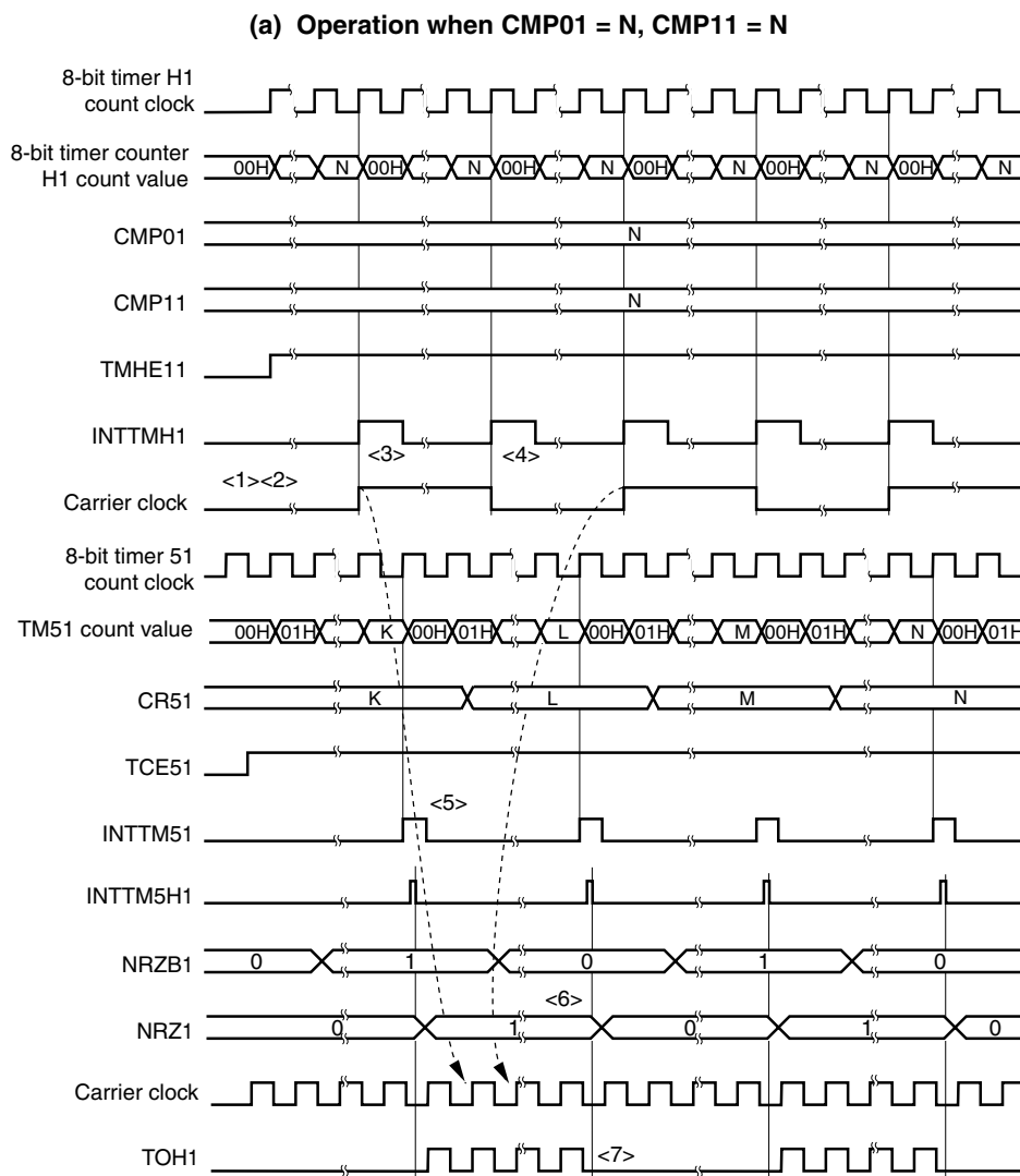
Figure 8-18. Carrier Generator Mode Operation Timing (1/3)
