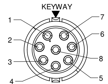
WIRE VIEW SHOWN 6282-8SG-3XX
