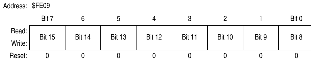
Figure 18-5. Break Address Register High (BRKH)
