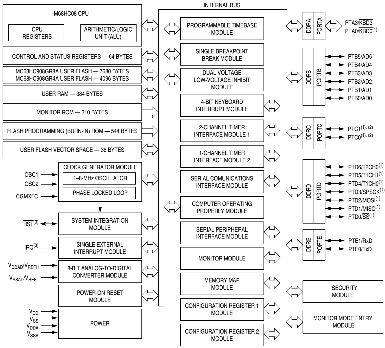
Figure 1-1 shows the structure of the MC68HC908GR8A.
