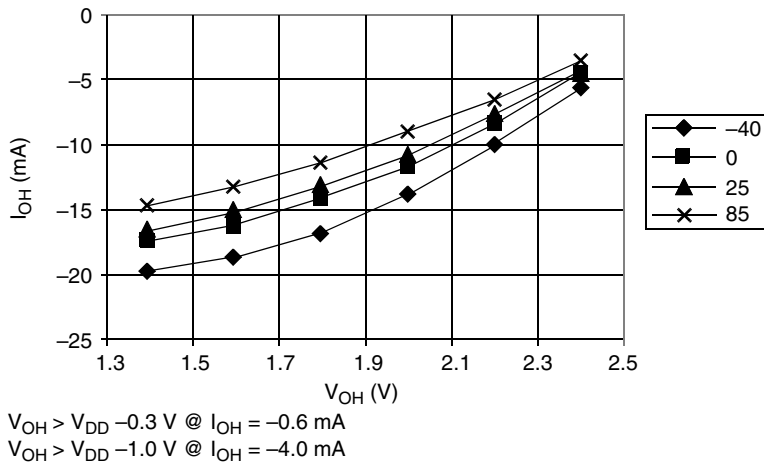
Figure 19-6. Typical High-Side Driver Characteristics — Ports PTB5–PTB0, PTD6–PTD0, and PTE1–PTE0 ( V_{DD} = 2.7 Vdc)
