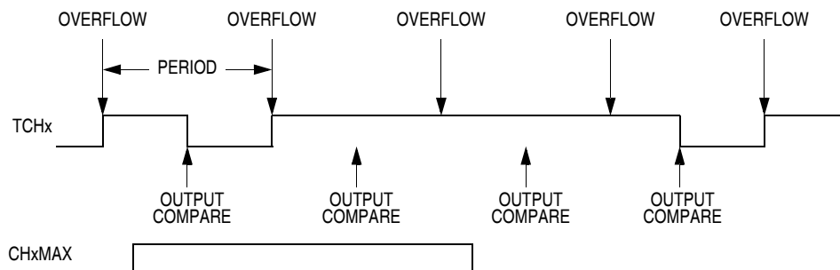
Figure 17-12. CHxMAX Latency
