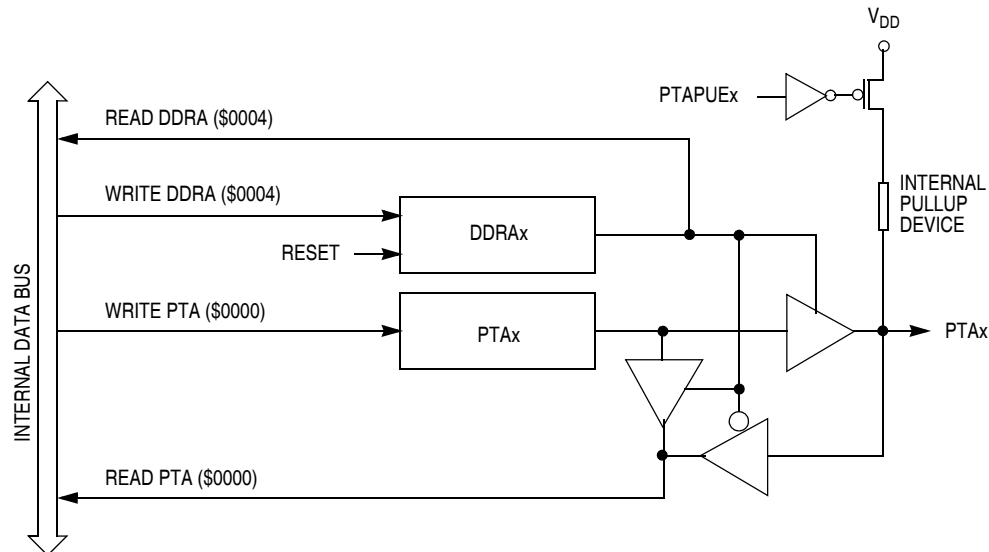
Figure 12-4. Port A I/O Circuit
