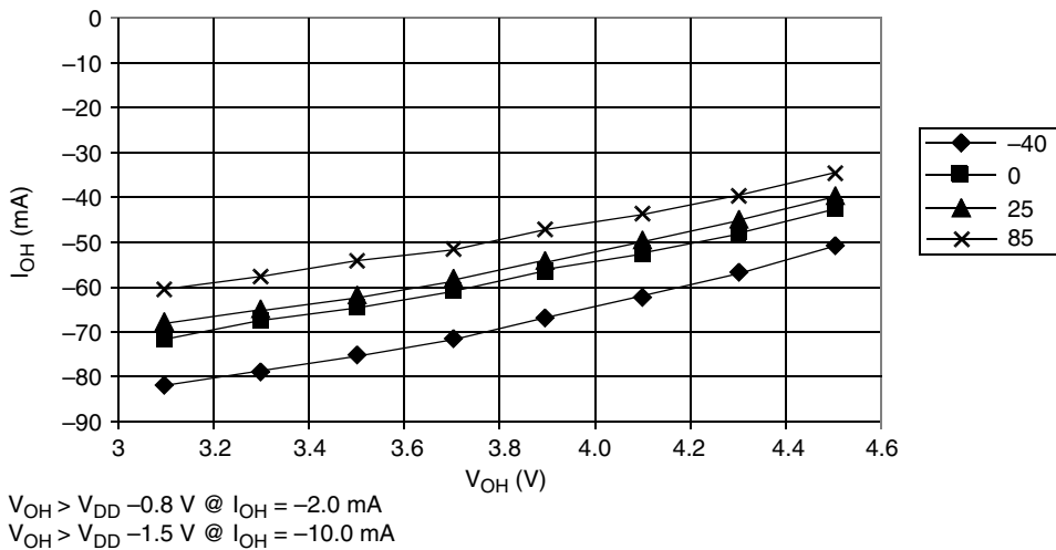
Figure 19-5. Typical High-Side Driver Characteristics — Ports PTB5–PTB0, PTD6–PTD0, and PTE1–PTE0 ( V_{DD} = 5.5 Vdc)
