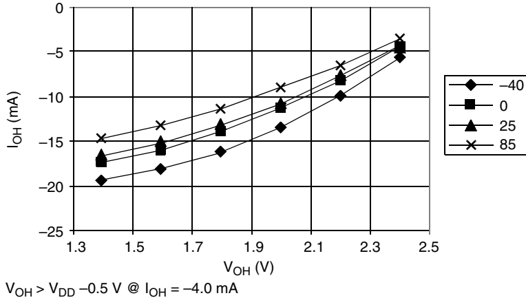
Figure 19-4. Typical High-Side Driver Characteristics — Port PTC1–PTC0 ( V_{DD} = 2.7 Vdc)
