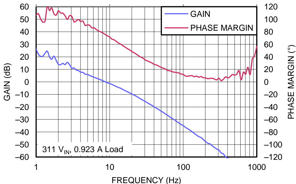
Figure 21. UCC28180EVM-573 Voltage Loop Response Gain and Phase, (162-V DC , full load, f CO = 8.6-Hz, phase margin = 63 degrees)
