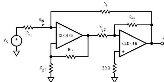
FIGURE 10. Composite Amplifier
