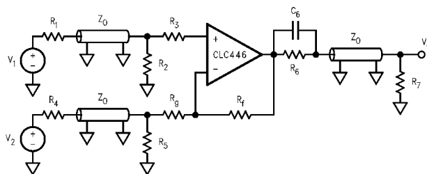
FIGURE 7. Transmission Line Matching
