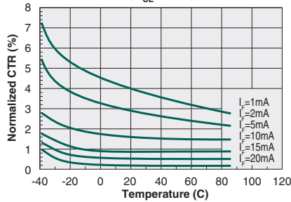
Single Transistor Normalized CTR vs. Temperature (V CE =0.5V)
