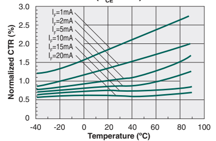
Typical Normalized CTR vs. Temperature (V CE =0.8V)
