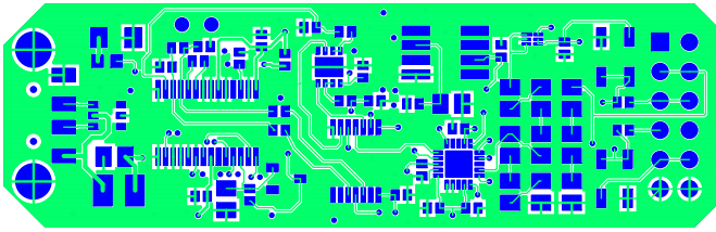
FIGURE 13. TOP LAYER
