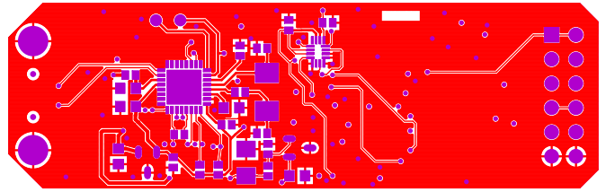
FIGURE 14. BOTTOM LAYER
