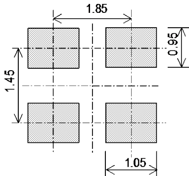
Fig.4 Land pattern
