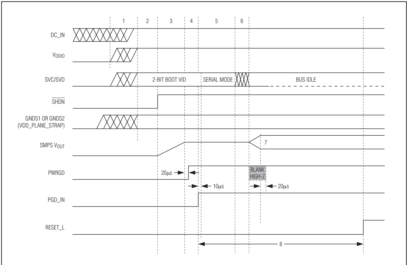
Figure 8. Startup Sequence
