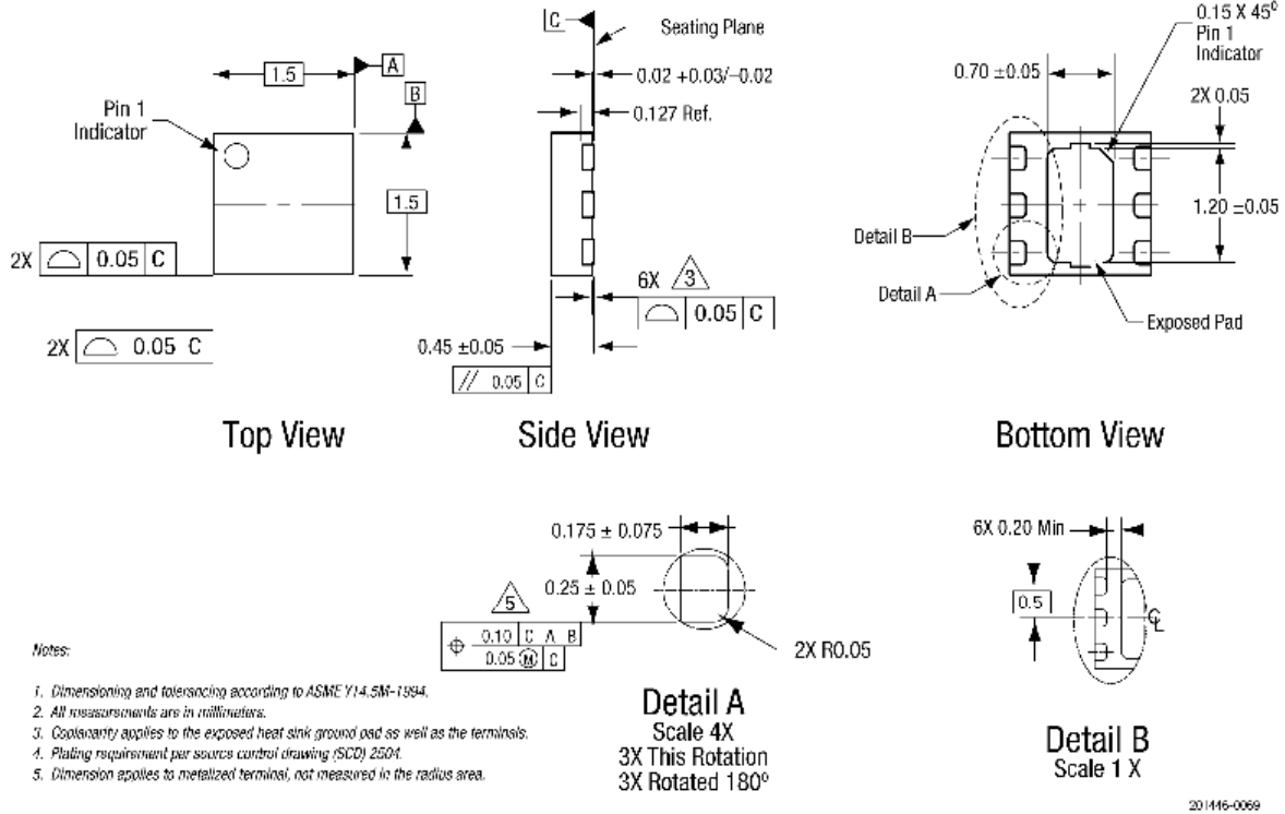
Figure 9. SKY65405-21 Package Dimensions
