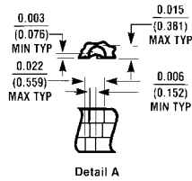
Ceramic Leadless Chip Carrier Package (E) Order Number 54LS20LMQB Package Number E20A
