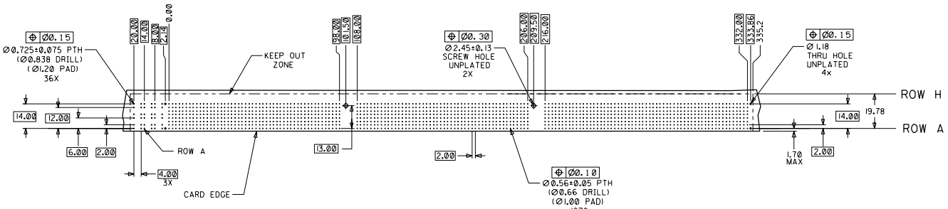
DAUGHTERCARD HOLE PATTERN (CONNECTOR SIDE)
