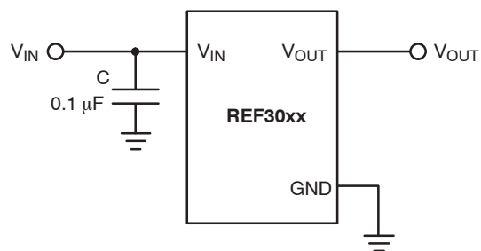
Figure 1. Application Circuit
