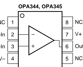
SO-8, 8-Pin DIP (OPA344 Only)
