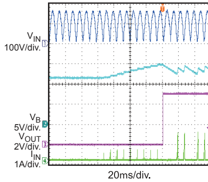
Thermal Shutdown Protection Recovery 115Vac
