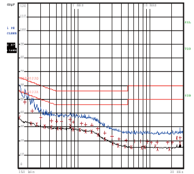
EMI Performance 230Vac, L Line
