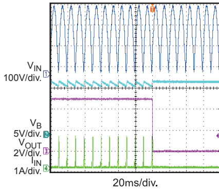
Thermal Shutdown Protection Entry 230Vac
