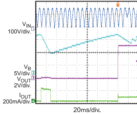
Short Circuit Protection Recovery 115Vac
