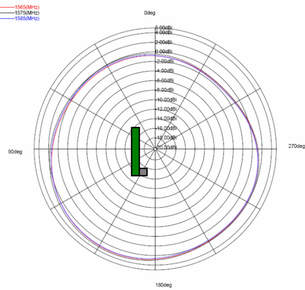
Figure 2: 1.575 GHz typical free space radiation patterns
