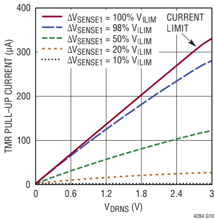
TMR Pull-Up Current vs DRNS Voltage
