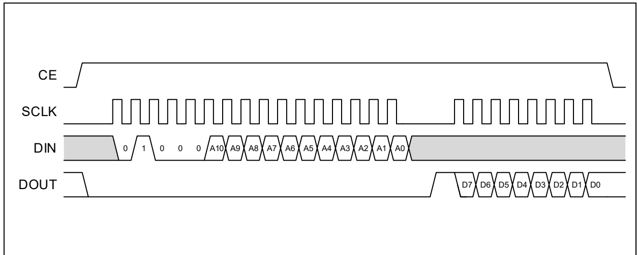
Figure 51: One-Byte Read
