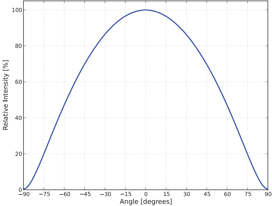
Figure 5. Typical radiation pattern for LUXEON 2835 with FreshFocus Technology at 120mA, T J =25°C.
