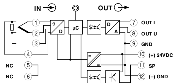
Figure 3 MCR-T-UI-E(-NC)
