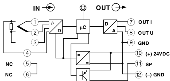
Figure 2 MCR-T-UI(-NC)
