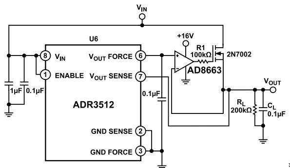
Figure 41. Boosted Output Current Reference
