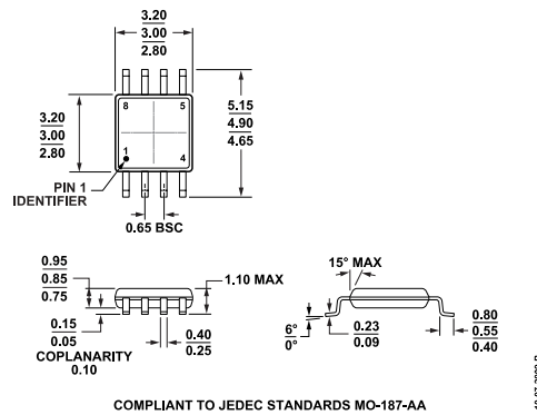
Figure 42. 8-Lead Mini Small Outline Package [MSOP] (RM-8)
