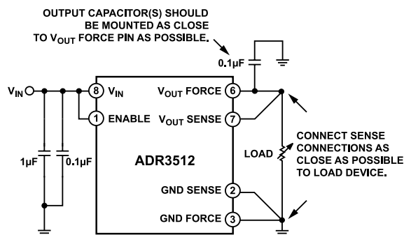
Figure 38. Application Showing Kelvin Connection
