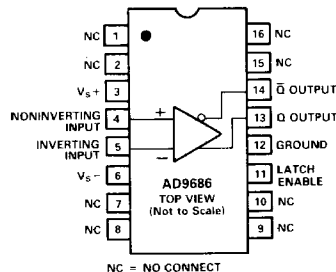
16-Pin DIP
