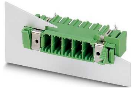
With threaded flange and shield feed-through on the inside of the device
