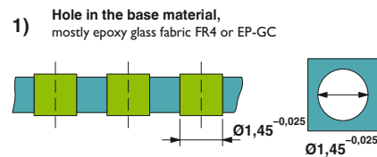
Structure of the metal-plated hole for EMC 1,5/...-G(F)-..., EMCV 1,5/...-G(F)-...
