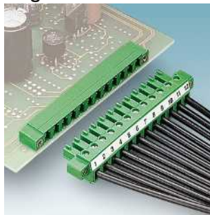
Plugs with screw connection and headers, 5.08 mm pitch MC 1,5/...-ST(F)-5,08 Page 246
