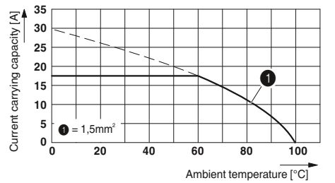
Current carrying capacity curve Type: SPT 1,5/5-3,5-H Test following DIN EN 60512-5-2:2003-01 Reduction factor = 1 No. of positions: 5
