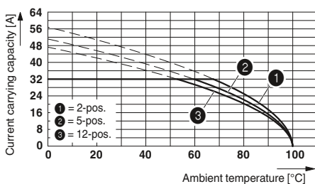
Type: ISPC 5/...-STGCL-7,62 with IPCV 5/...-G-7,62
