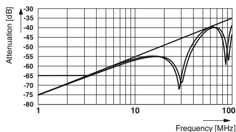
Near end crosstalk attenuation for PTPM plug with Ethernet cable
