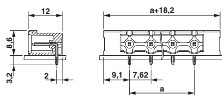
Drilling diagram
