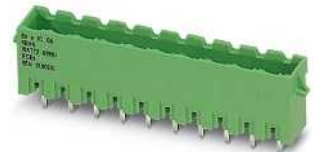
With engagement noses, plug-in direction vertical to the PCB
