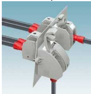
RW 8 series: bolt connection, up to 125 A, connection: vertical and horizontal RW 8... Page 626
