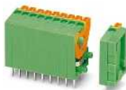
2.54 mm pitch, with opening lever, conductor connection vertical to the PCB
