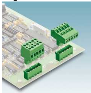
TWIN plugs, 5.08 mm pitch, for potential distribution TMSTBP 2,5/...-ST(F)-5,08 Page 270
