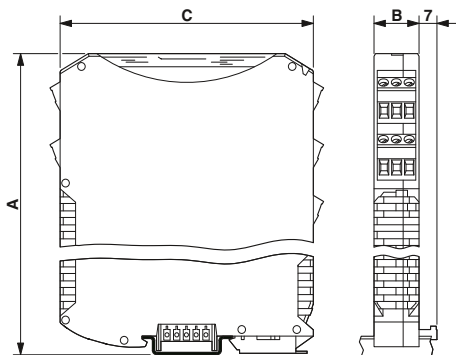
A = 114.5 mm; B = 35 mm; C = 99 mm,
