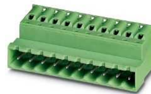
Inverted plug with push-in spring connection, with screwdriver actuation shaft, and test connection
