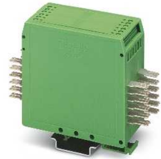
12- and 24-pos. with slotted 6.3/2.8 mm slip-on connection, width: 40 mm
