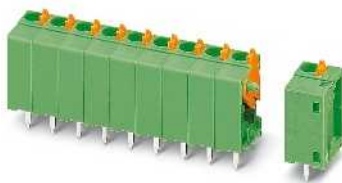
5.08 mm pitch, with shortened opening lever, conductor connection vertical to the PCB
