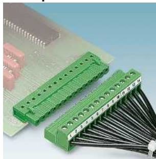
Inverted plug with screw connection, 5.08 mm pitch IC 2,5/...-ST(F)-5,08 Page 272
