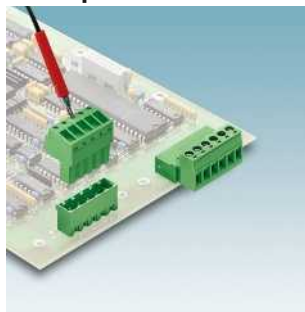
Plugs with screw connection, 5.0/5.08 mm pitch, with/without test connection MSTB 2,5/...-ST(F)... Page 262
