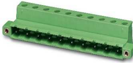
With threaded flange for screw connection using GMSTB connectors
