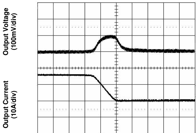
Figure 5. Transient Load Response (typical V_{in} , load current steps from 50% to 25% at a slew rate 0.1A/ \mu s)
