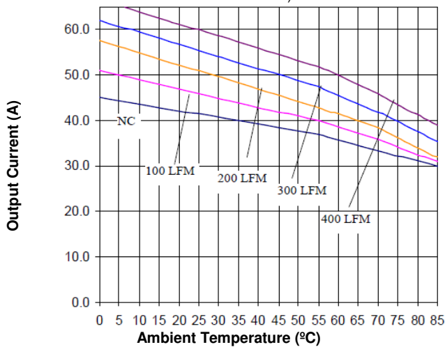
Figure 11. Current Derating Curve for Airflow Direction 3 (Ref. Fig. 10 for Airflow Direction; typical V_{in} with baseplate, soldered interface)
