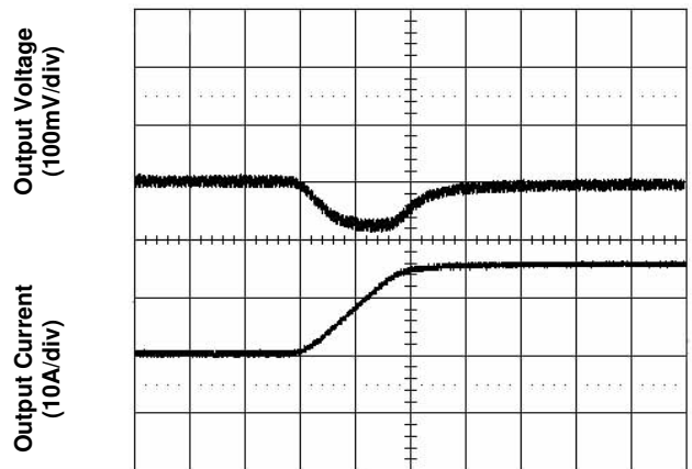
Figure 6. Transient Load Response (typical V_{in} , load current steps from 50% to 75% at a slew rate 0.1A/ \mu s)
