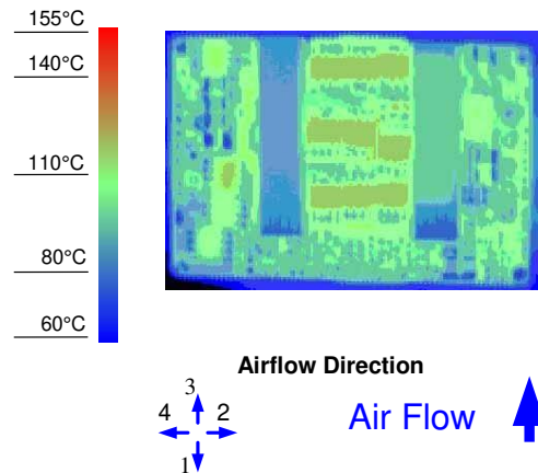
Figure 10. Thermal Image for Airflow Direction 3 (46.5A output, 55°C ambient, 200 LFM, typical V_{in} , open frame, soldered interface)
