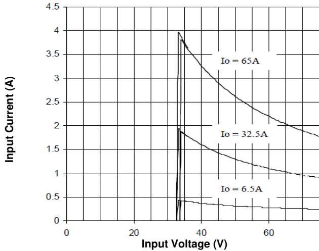
Figure 7. Input Characteristics
