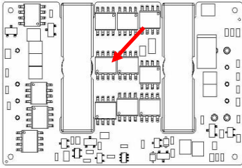
Figure 17. Temperature Monitoring Locations
