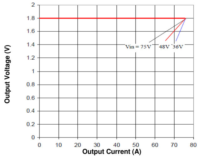
Figure 8. Output Characteristics
