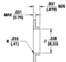
Mounting Holes
