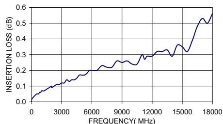
141-6SM+ INSERTION LOSS
