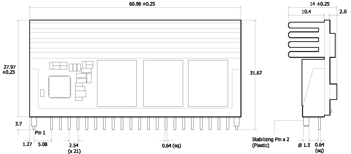
Figure 14. Mechanical Drawing
