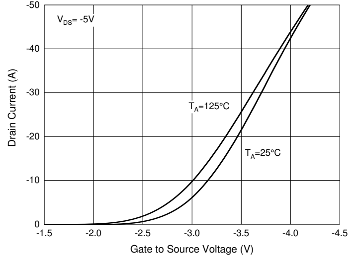
Fig. 2 - Transfer Characteristics
